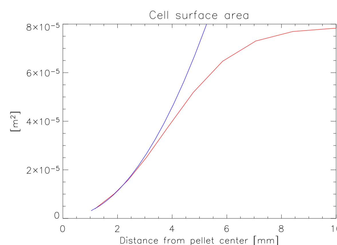
Figure 2. An illustration of the analytic transition from spherical expansion to channel flow - plot of the dependence of the cell surface area as a function of the distance from the pellet center. Blue curve - spherical expansion, red curve - spherical expansion turning into channel flow.
