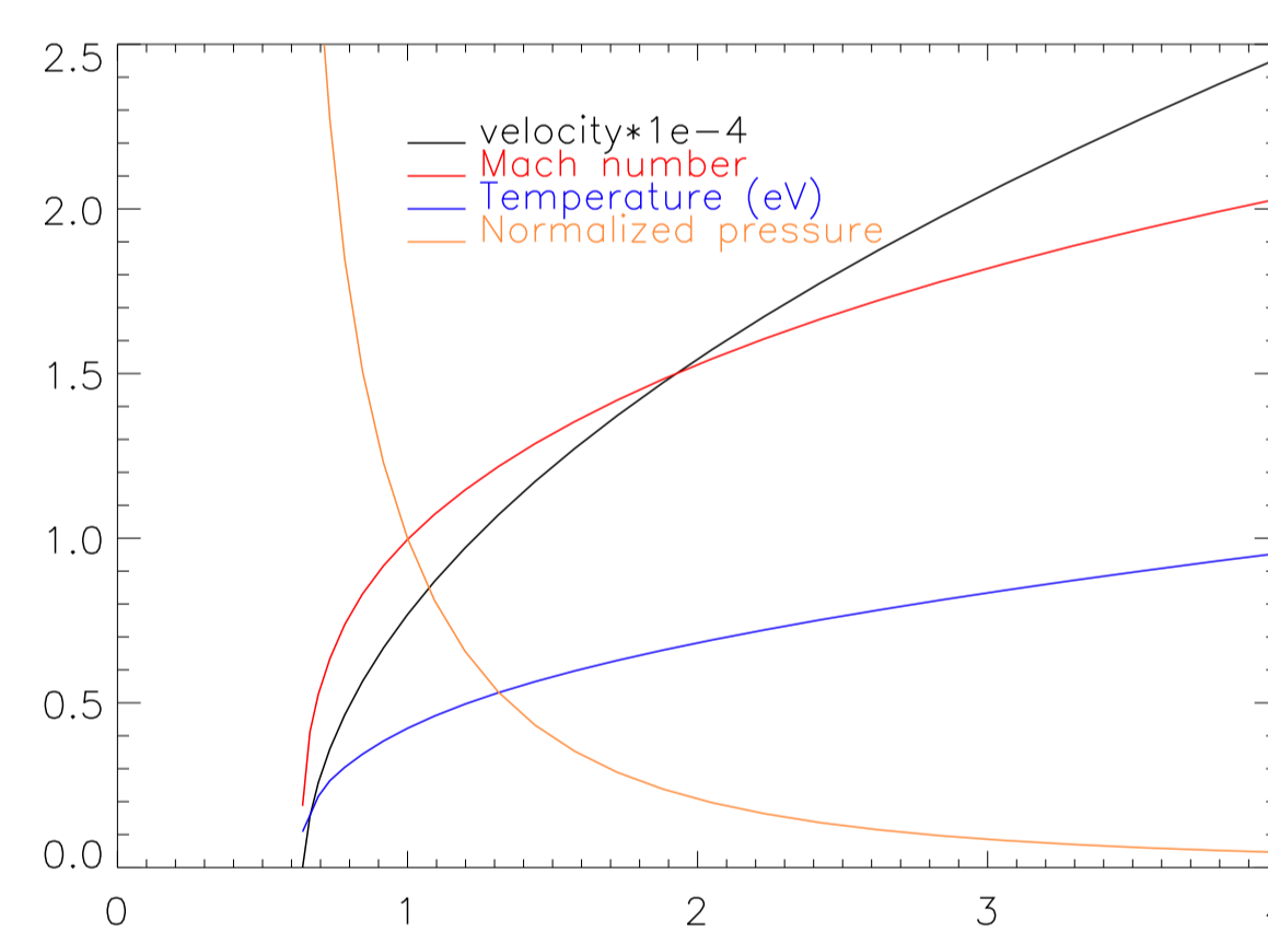
Figure 3. The normalized pressure in the cells, the cells' temperature, the Mach number of the cells' expansion, and the expansion velocity as a function of the distance from the pellet center in units of the position of the sonic surface.
