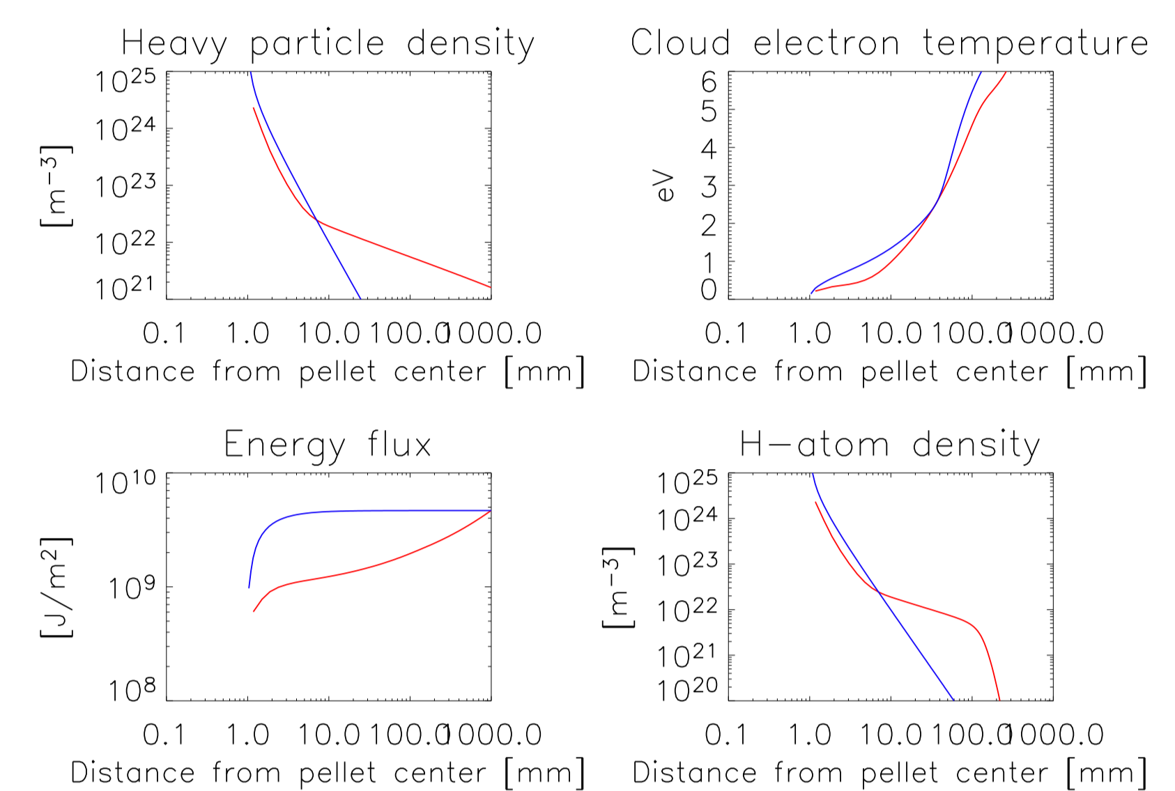
Figure 4. The comparison of the model's results for pure spherical expansion (blue curve) and spherical expansion turning into channel flow (red curve).
