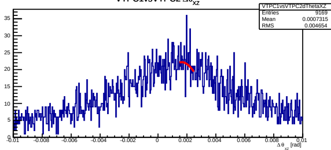
VTPC1vsVTPC2 \Delta\theta_{xz}
