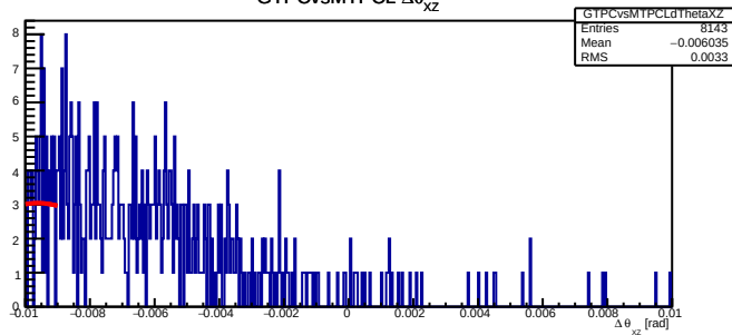
GTPCvsMTPCL \Delta\theta_{xz}
