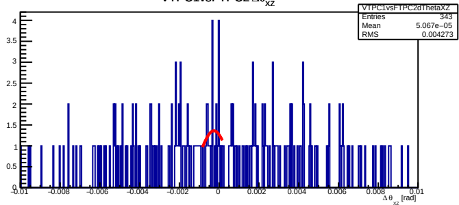
VTPC1vsFTPC2 \Delta\theta_{xz}
