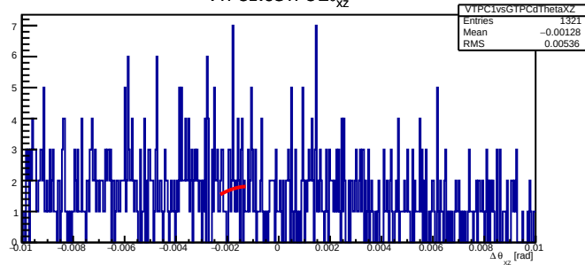
VTPC1vsGTPC \Delta\theta_{xz}
