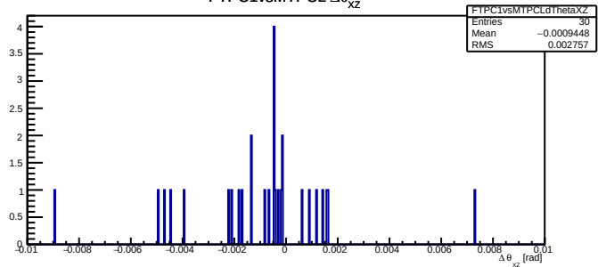
FTPC1vsMTPCL \Delta\theta_{xz}
