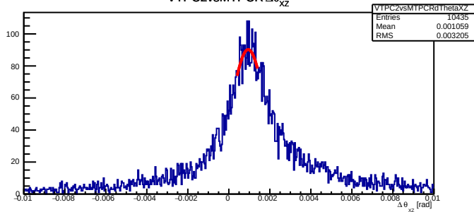
VTPC2vsMTPCR \Delta\theta_{xz}
