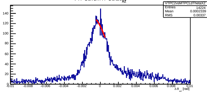
VTPC2vsMTPCL \Delta\theta_{xz}
