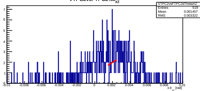
VTPC2vsFTPC2 \Delta\theta_{xz}
