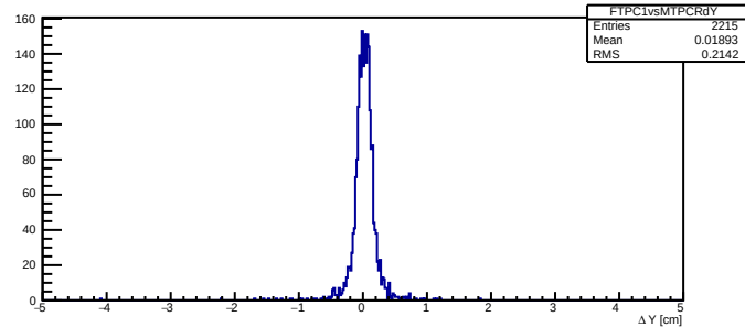
FTPC1vsMTPCR \Delta Y
