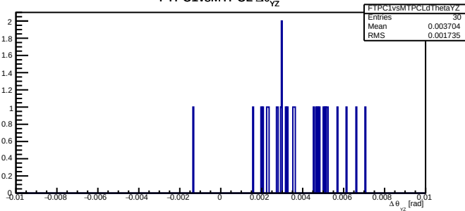
FTPC1vsMTPCL \Delta\theta_{yz}
