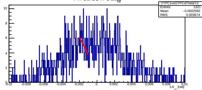
VTPC1vsGTPC \Delta\theta_{yz}
