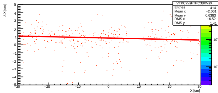
VTPC2vsFTPC3 \Delta X vs. X
