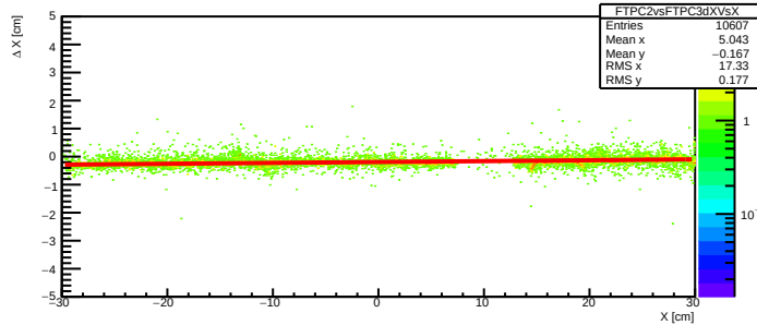
FTPC2vsFTPC3 \Delta X vs. X
