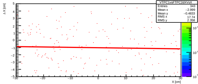
VTPC1vsFTPC2 \Delta X vs. X
