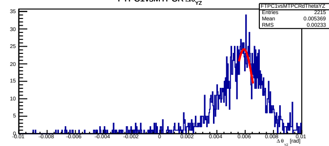
FTPC1vsMTPCR \Delta\theta_{yz}
