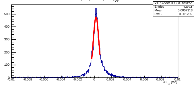
VTPC2vsMTPCL \Delta\theta_{yz}
