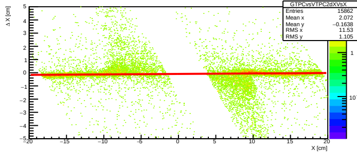
GTPCvsVTPC2 \Delta X vs. X
