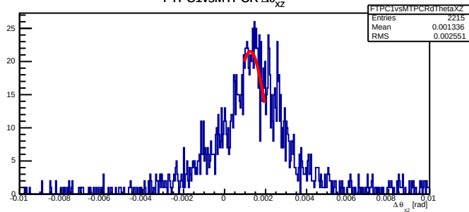
FTPC1vsMTPCR \Delta\theta_{xz}
