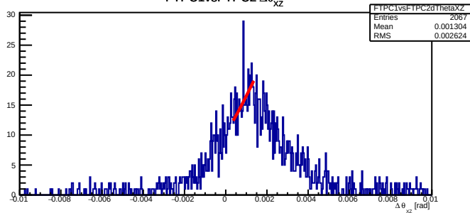
FTPC1vsFTPC2 \Delta\theta_{xz}
