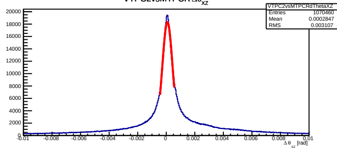
VTPC2vsMTPCR \Delta\theta_{xz}
