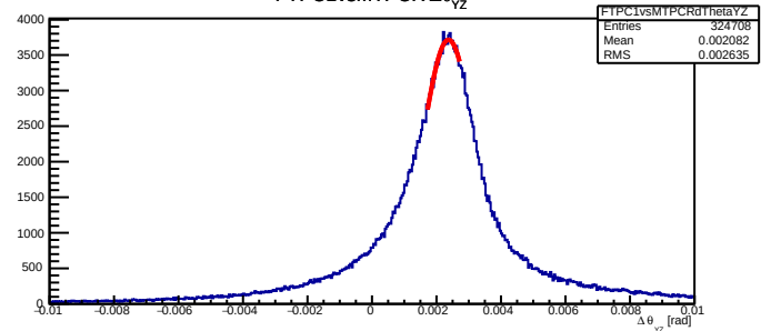
FTPC1vsMTPCR \Delta\theta_{yz}
