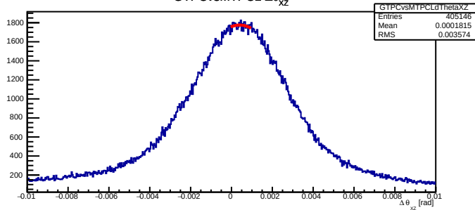
GTPCvsMTPCL \Delta\theta_{xz}
