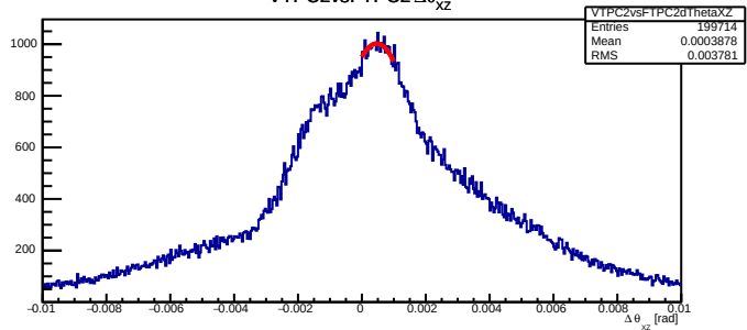
VTPC2vsFTPC2 \Delta\theta_{xz}
