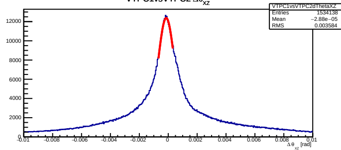
VTPC1vsVTPC2 \Delta\theta_{xz}
