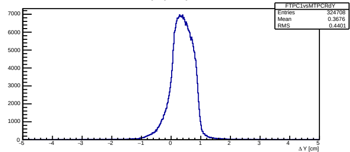
FTPC1vsMTPCR \Delta Y
