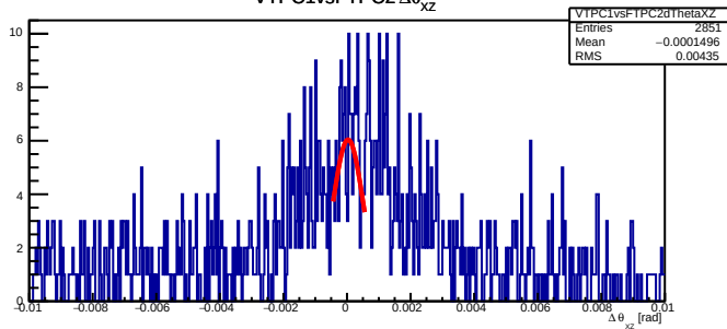
VTPC1vsFTPC2 \Delta\theta_{xz}
