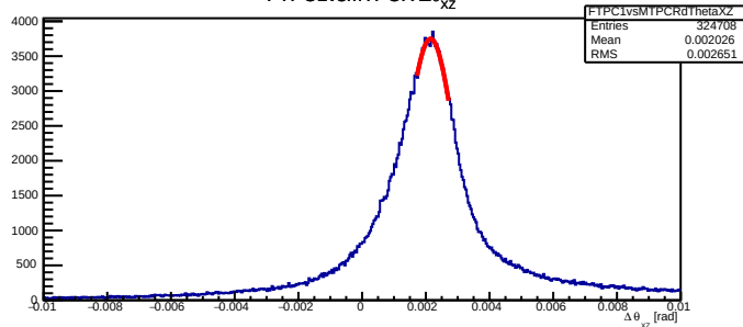
FTPC1vsMTPCR \Delta\theta_{xz}
