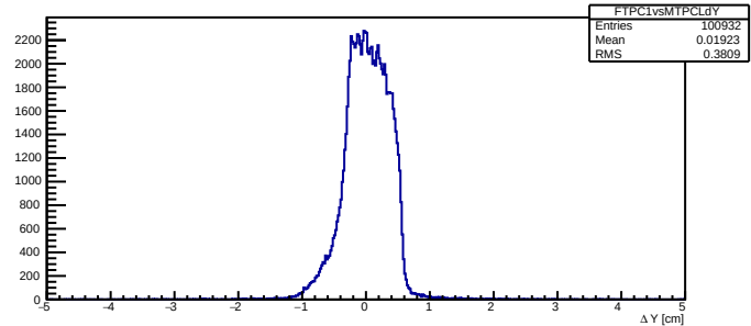
FTPC1vsMTPCL \Delta Y
