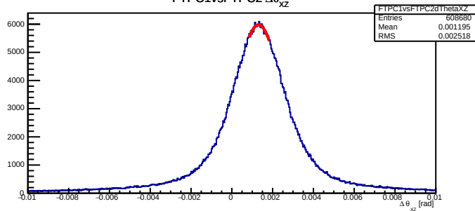
FTPC1vsFTPC2 \Delta\theta_{xz}
