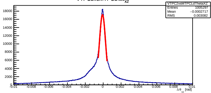
VTPC2vsMTPCL \Delta\theta_{xz}
