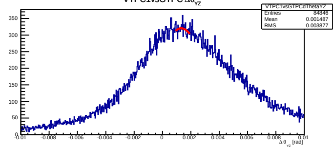
VTPC1vsGTPC \Delta\theta_{yz}
