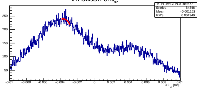
VTPC1vsGTPC \Delta\theta_{xz}
