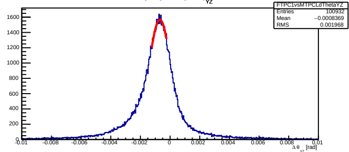
FTPC1vsMTPCL \Delta\theta_{yz}
