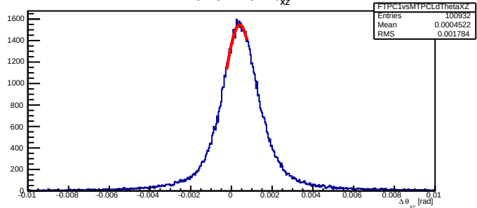
FTPC1vsMTPCL \Delta\theta_{xz}
