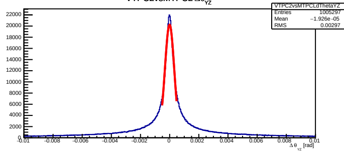
VTPC2vsMTPCL \Delta\theta_{yz}
